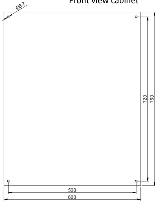
Front view cabinet
